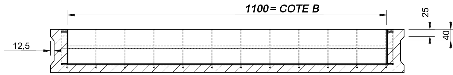
Section B-B
